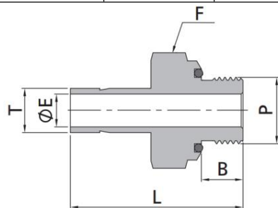
Fractional Tube to SAE/MS Thread
