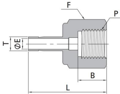
Metric Tube to ISO Parallel Thread
