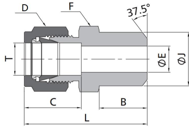
Metric Tube to Pipe Butt Weld
