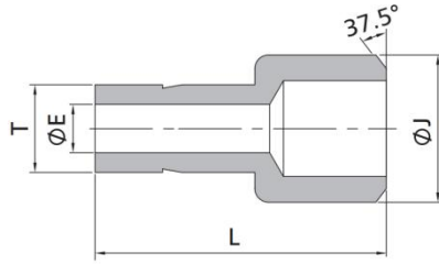
Fractional Tube to Pipe Weld
