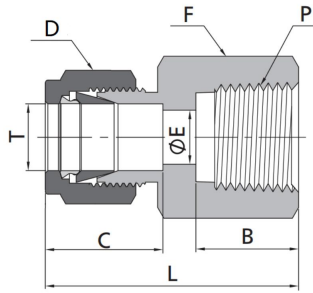
Metric Tube to NPT Thread
