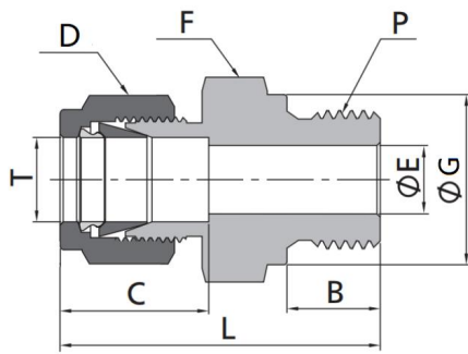
Metric Tube to ISO Parallel Thread
