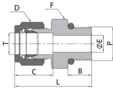
Fractional Tube to SAE/MS Thread
