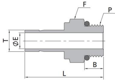
Fractional Tube to SAE/MS Thread
