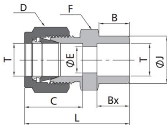
Metric Tube to Tube Socket Weld
