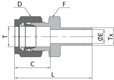
Metric Tube to Fractional Tube
