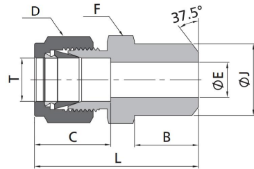
Fractional Tube to Pipe Butt Weld
