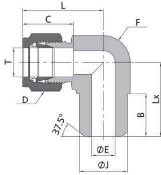
Fractional Tube to Pipe Butt Weld
